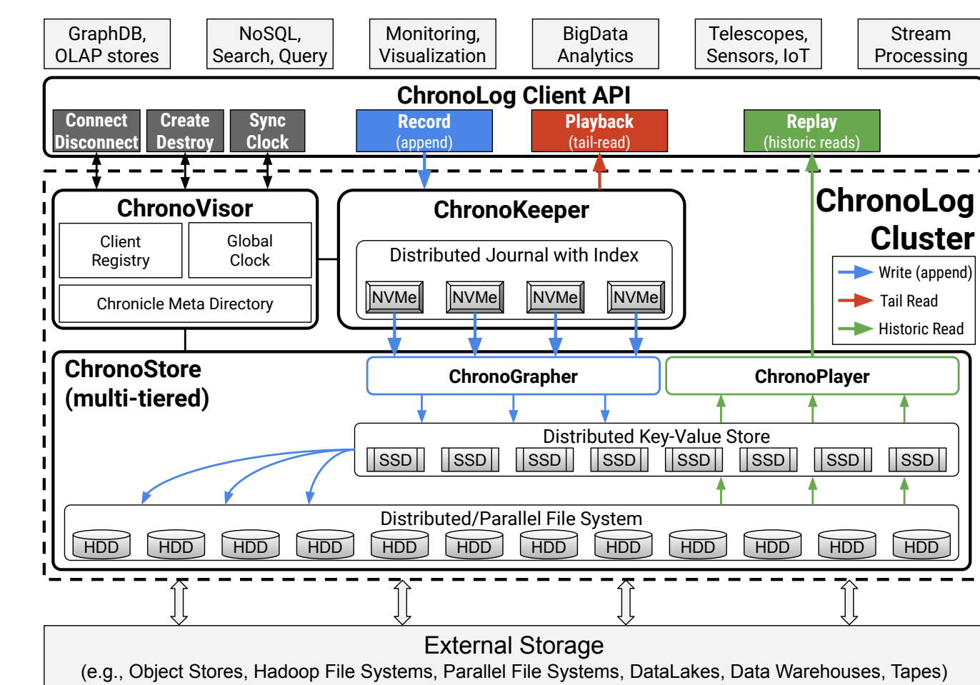
Figure 3: Chronolog design
