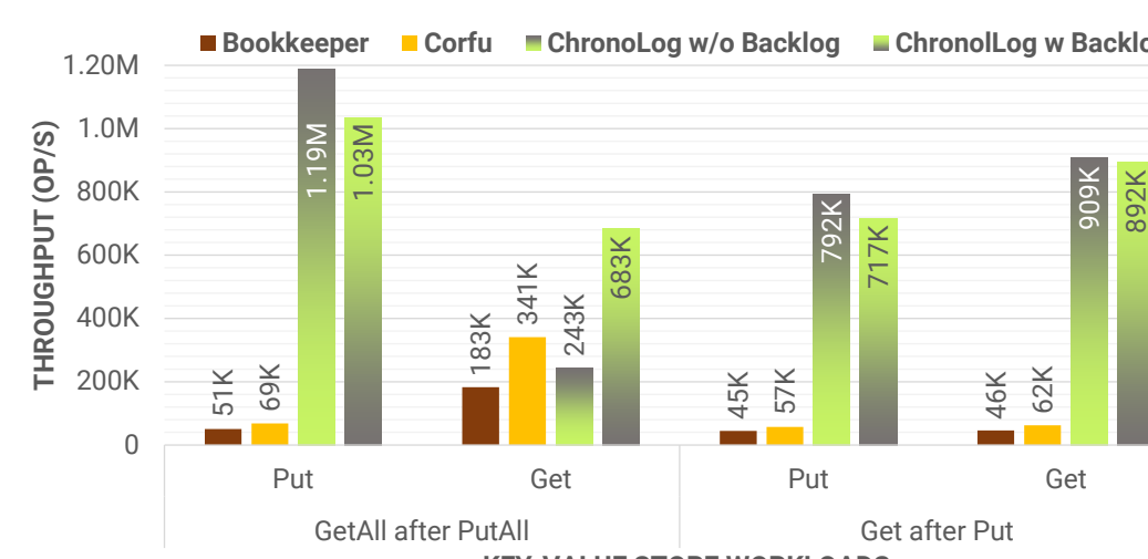
Figure 7: ChronoLog backend for KVS
