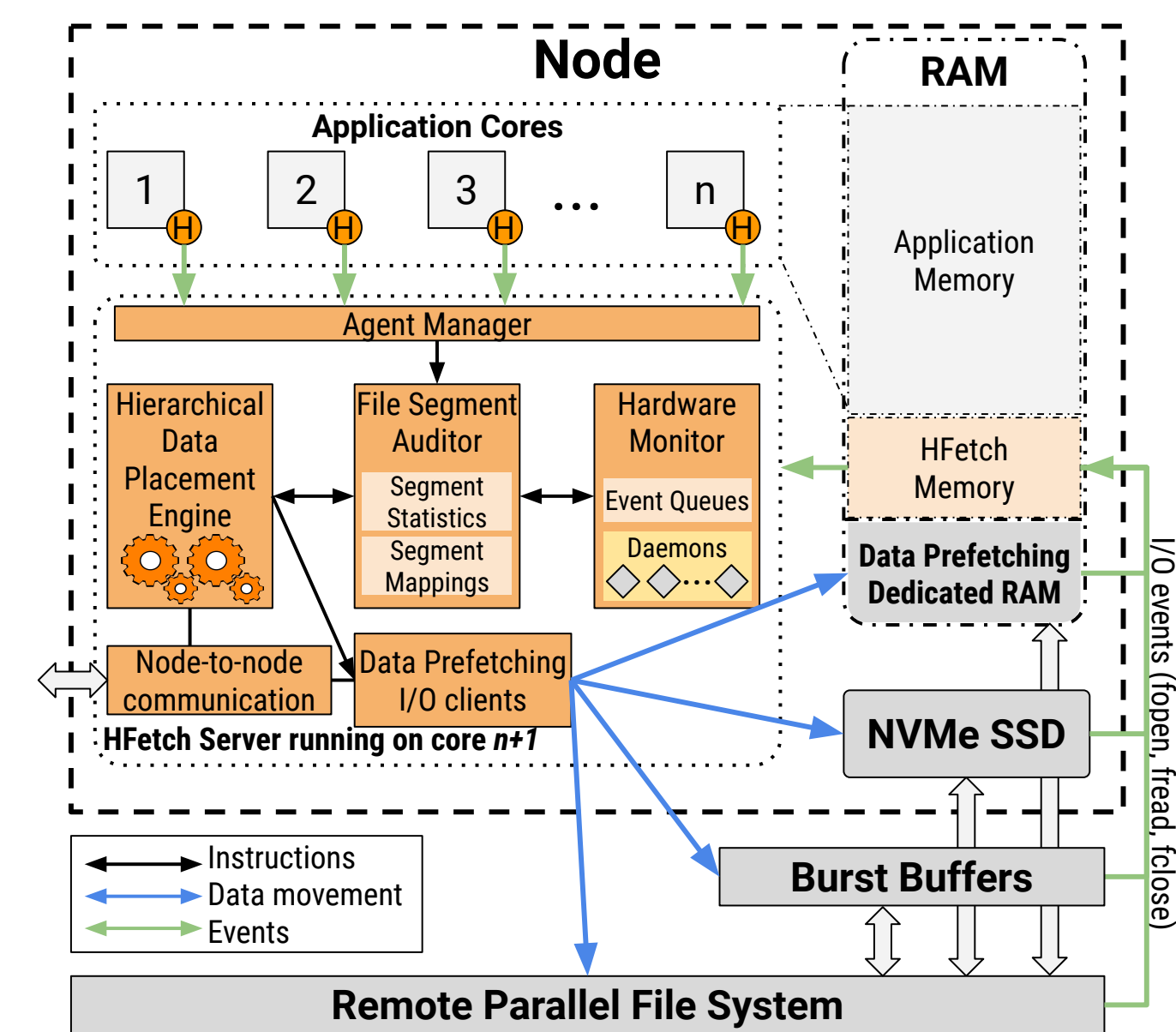
Figure 5: HFatch design
