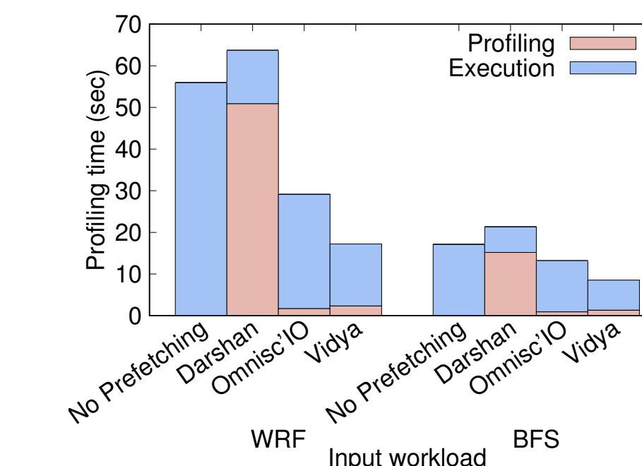
Figure 6: Vidya: Prefetching On/Off
