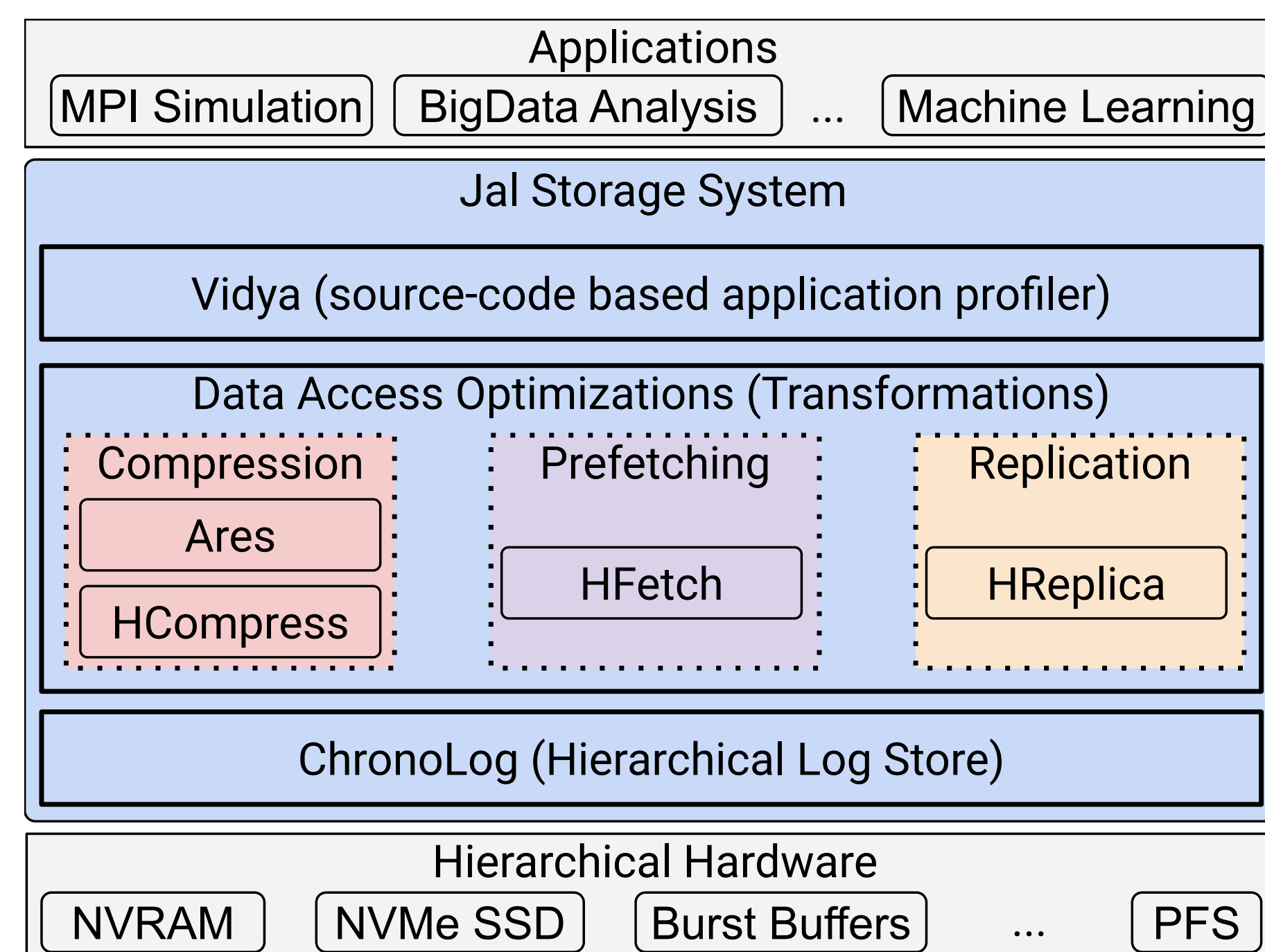
Figure 1: High-Level architecture of Jal Storage System
