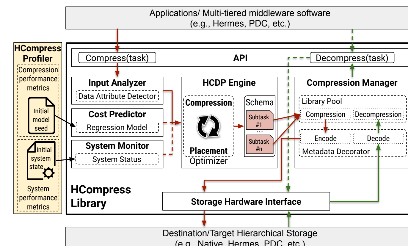
Figure 4: HCompress design
