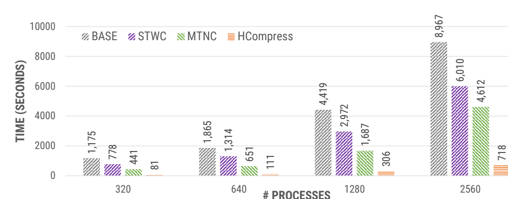
Figure 8: HCompress: Scientific workflow
